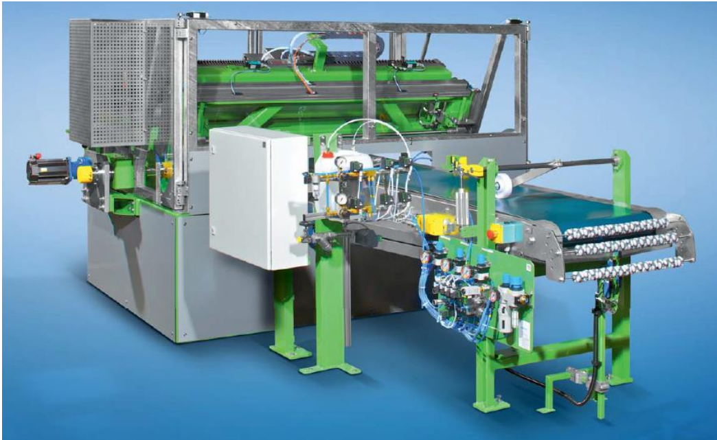
Slika 19 – Troester Tread Cutting Machine
